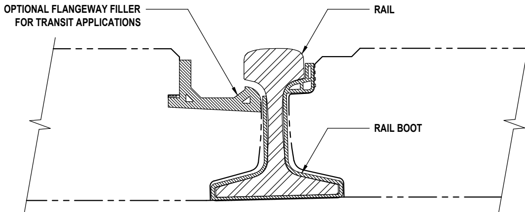
RAIL WITH BOOT & FLANGEWAY FILLER
