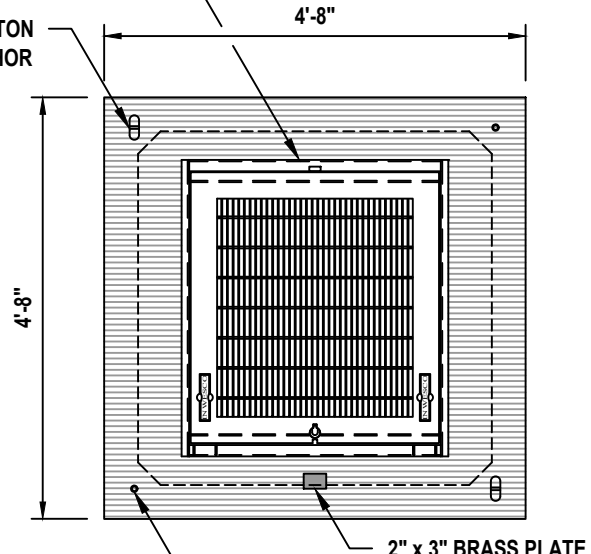
TOP PLAN
