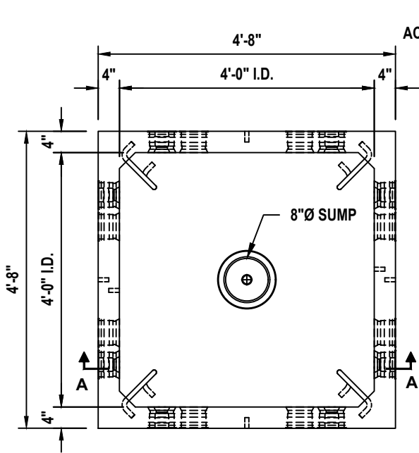
PLAN VIEW TOP NOT SHOWN, SEE TOP PLAN
