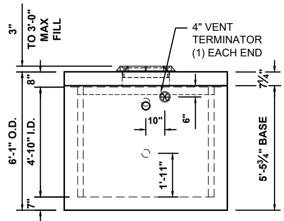
VIEW-B
