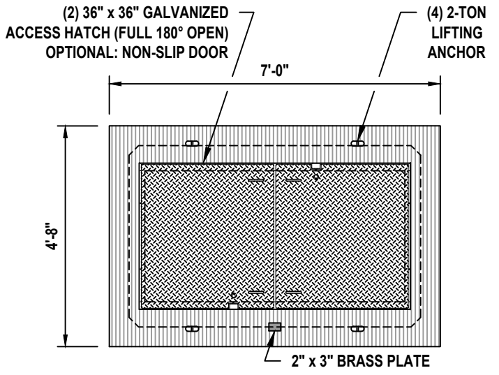
TOP PLAN
